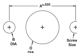
Panel Hole Sizes Medium Pressure Needle Valve Panel Mount
