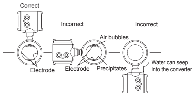
Mounting Orientation
