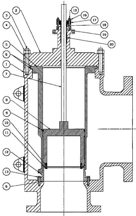
Figure 1 – Hung Cage Construction
