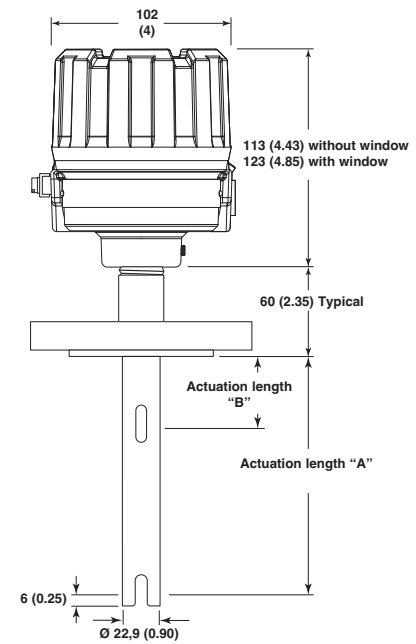
962 - Flanged connection
